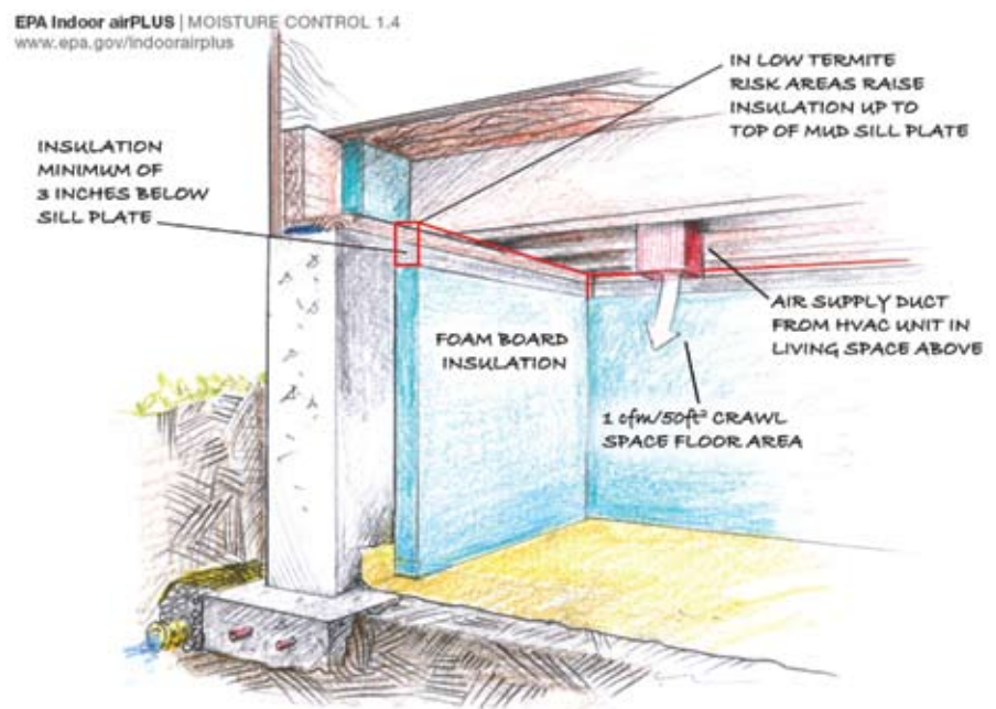
Figure 3. Sketch of a closed crawl space with conditioned air supply. [Illustration: Dennis Livingston, Community Resources. Reprinted with permission of the U.S. Environmental Protection Agency.]
